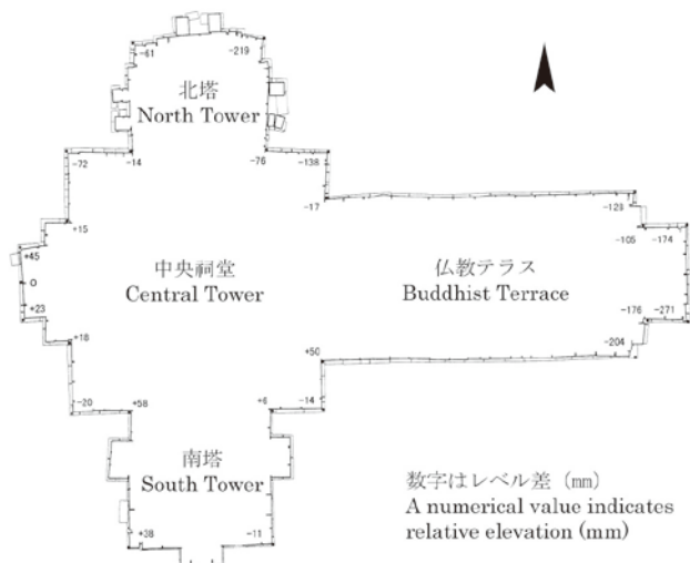
下成基壇延石・地覆石平面図 (S=1/400) Plan of foundation stones for the first tier platform (S=1/400)
