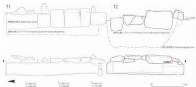
サブトレンチT1・T2における掘込地業内石列の断面図（上）と平面図（下） Cross-section (above) and plane view (below) of the lines of stones inside the basement at the sub-trench of T1 and T2
