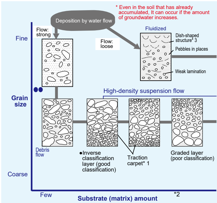
Figure 4. Image of sediment concentration and particle size (facies are different depending on water volume and flow will be different)
